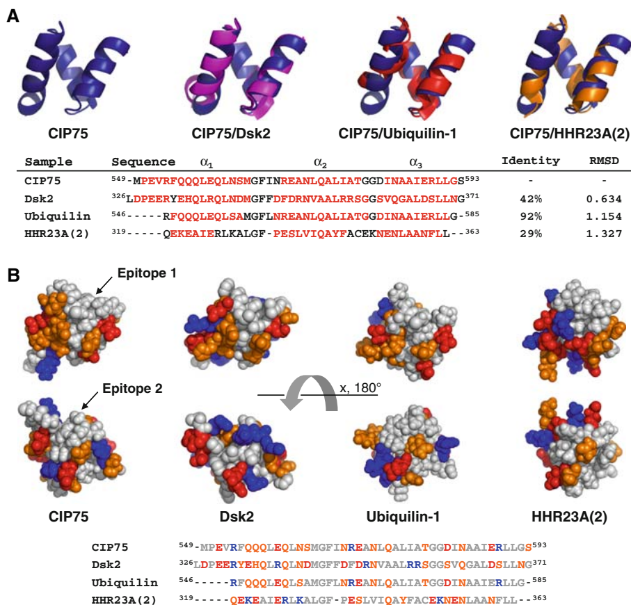
Fig. 2 Comparison of the CIP75 UBA domain structure with previously solved UBA domains. A. Presented is the ribbon diagram structure of the CIP75 UBA domain alone and aligned with the UBA domains from Dsk2 (PDB: 2BWB) (purple), Ubiquilin-1 (PDB: 2JY5) (red), and HHR23A(2) (PDB: 1DV0) (orange). Below the structures is an alignment of their sequences, with the percent identity and RMSD compared with the CIP75 UBA domain. The RMSD is for alignment of the backbone atoms. Residues comprising the three
