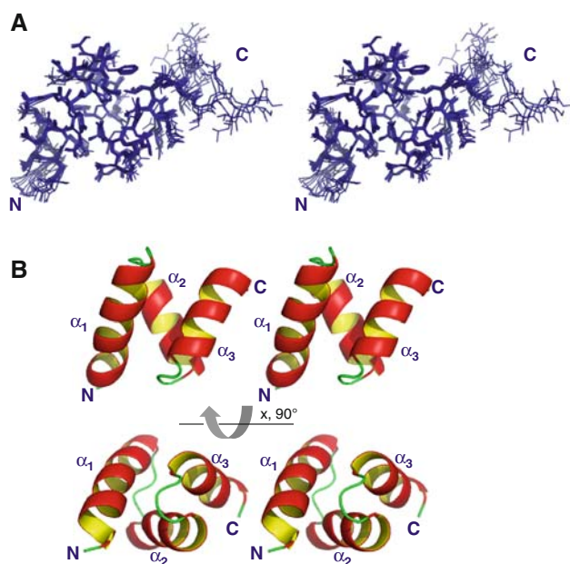
Fig. 1 Solution structure of the UBA domain of CIP75. A. Stereoview of the 10 lowest energy structures which have been superposed according to the backbone atoms (region M549-S593). B. Stereoview of the ribbon diagram of the lowest energy CIP75 UBA domain structure. The three \alpha -helices ( \alpha_1 , \alpha_2 , and \alpha_3 ) and the amino (N) and carboxyl (C) terminal domains have been labeled
